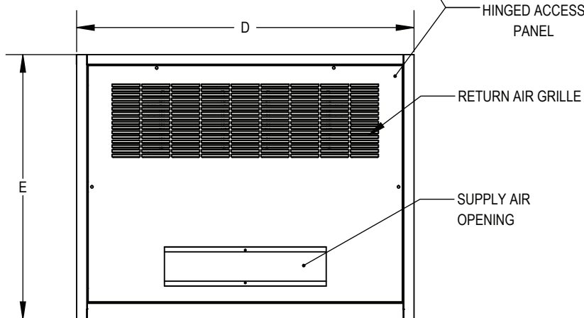
BOTTOM VIEW
