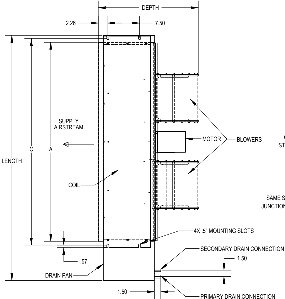
TOP VIEW
